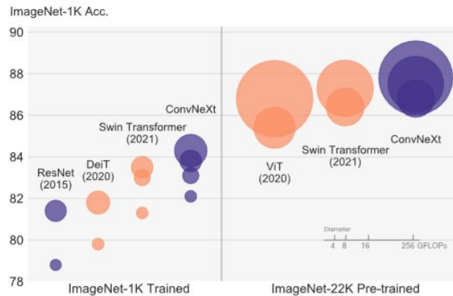
Figure 1. ImageNet-1K classification results for ● ConvNets and ○ Vision Transformers.
